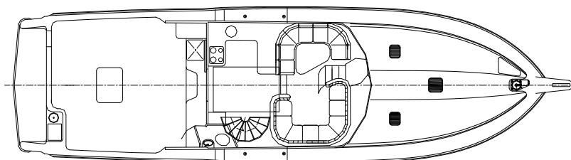
SALOON AND COCKPIT DECK PLAN
